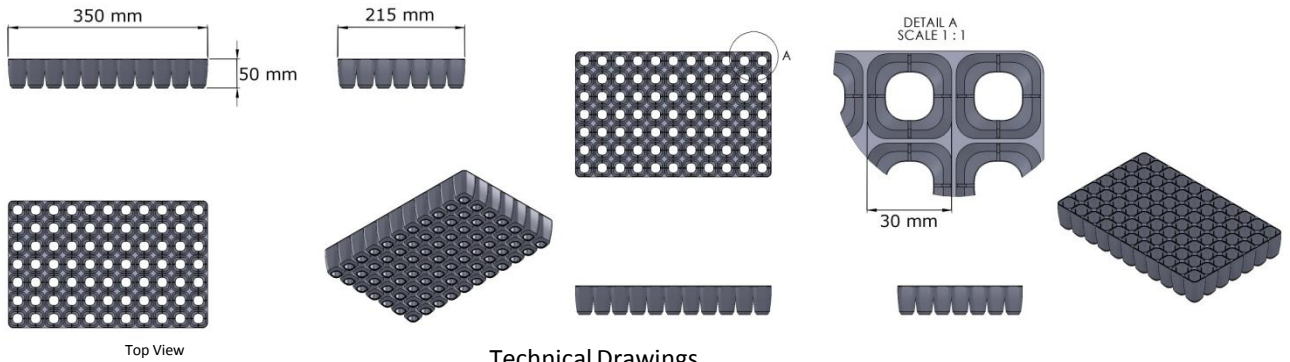
Technical Drawings
