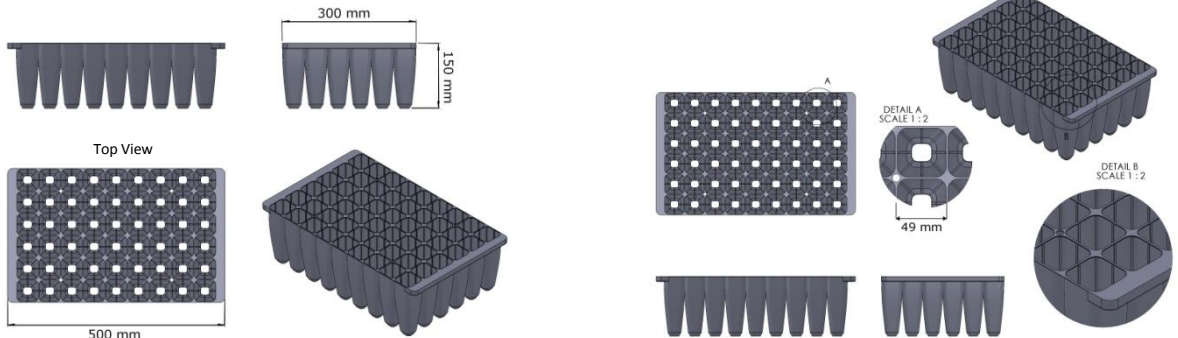
Technical Drawings
