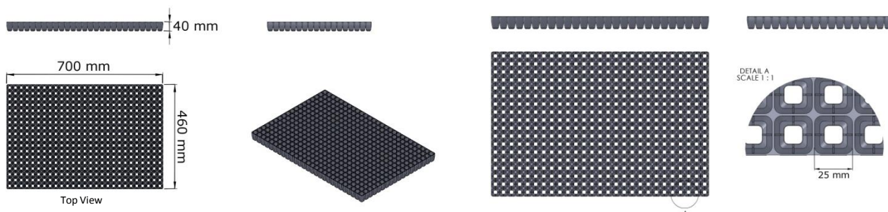
Technical Drawings
