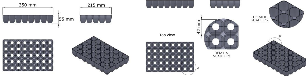
Technical Drawings
