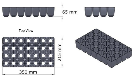
Technical Drawings
