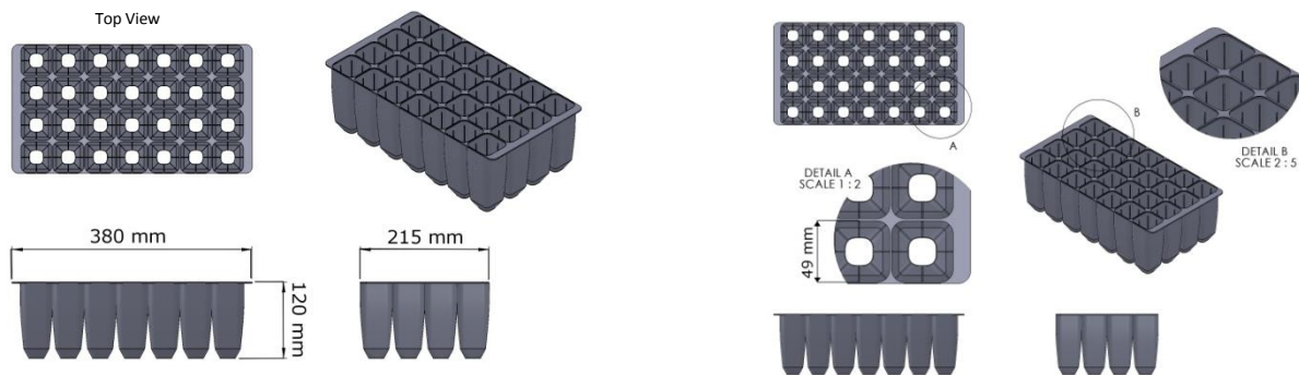
Technical Drawings
