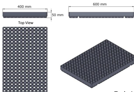
Technical Drawings
