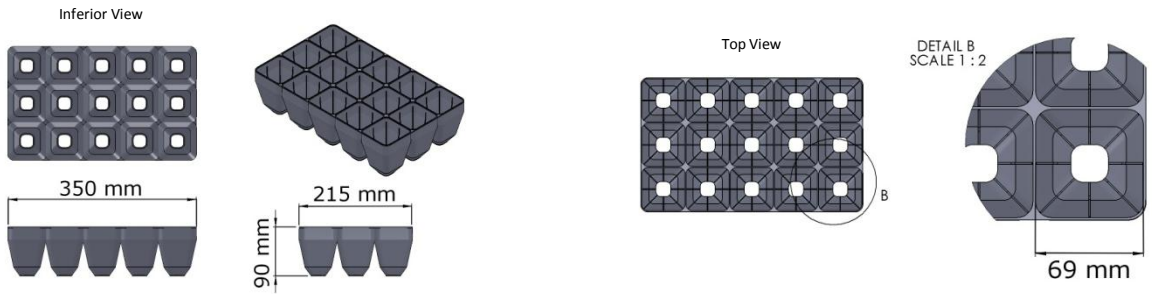
Technical Drawings
