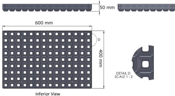
Technical Drawings
